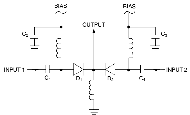
C 2 , C 3 — Chip MIS capacitor C 1 , C 4 — Chip or beam — lead MIS capacitor D 1 , D 2 DSG9500 beam — lead pIN diode
